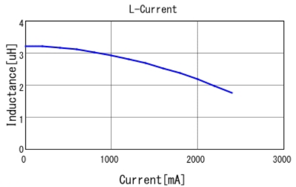
■ 1269AS-H-3R3M L-Current 20degC
